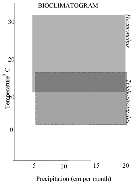
Figure 2 A bioclimatogram showing average temperature and rainfall conditions which are favourable for the development of Haemonchus (top) and Trichostrongylus (bottom) infective larvae.
